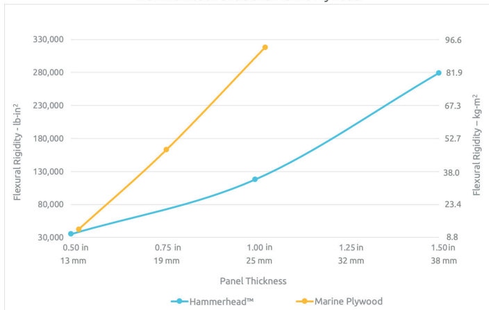
Thickness and Rigidity Comparison Hammerhead Panels and Marine Plywood
