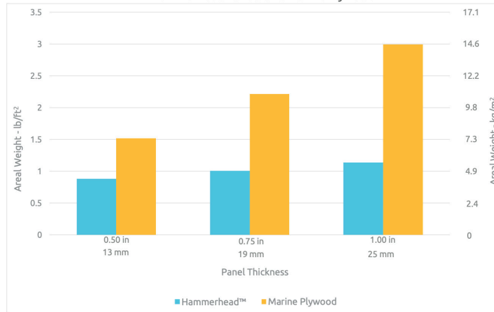
Weight to Thickness Comparison Hammerhead Panels and Marine Plywood
