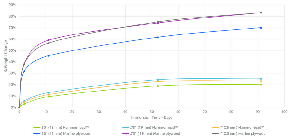
Moisture Absorption Comparison Hammerhead Panels and Marine Plywood % weight change due to water absorption
