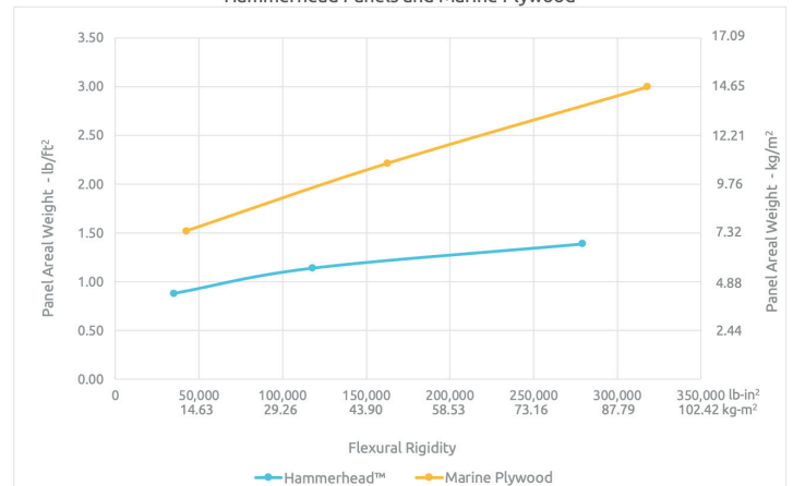
Weight to Rigidity Comparison Hammerhead Panels and Marine Plywood
